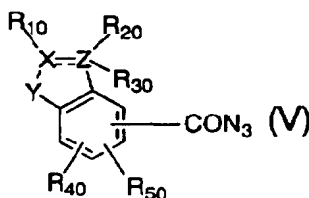
Formula (V)
